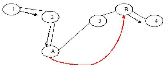
Figure 1: A wormhole attack performed by colluding malicious nodes A and B.
